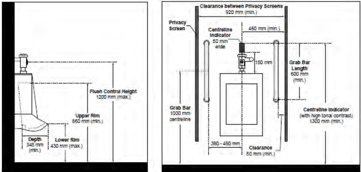
Figure 25: Urinal spacing requirements
