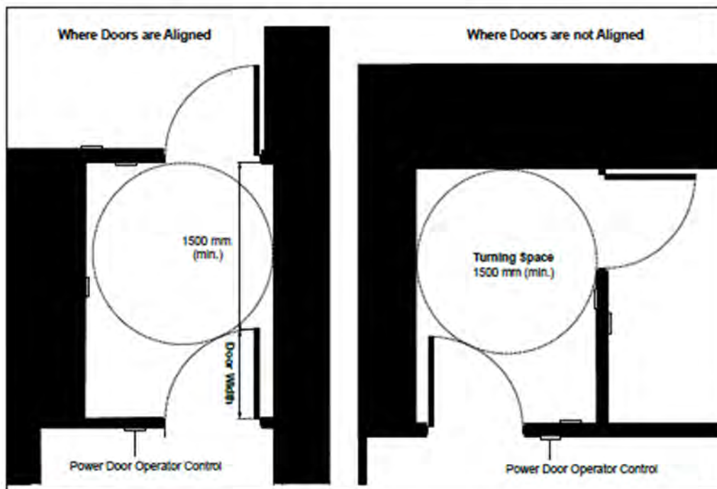
Figure 13: Turning radius between doors
