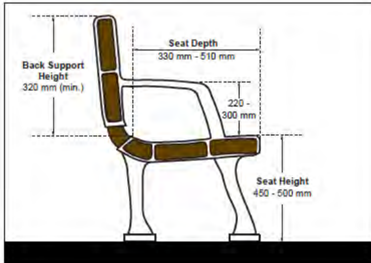
Figure 35: Chair dimension requirements
