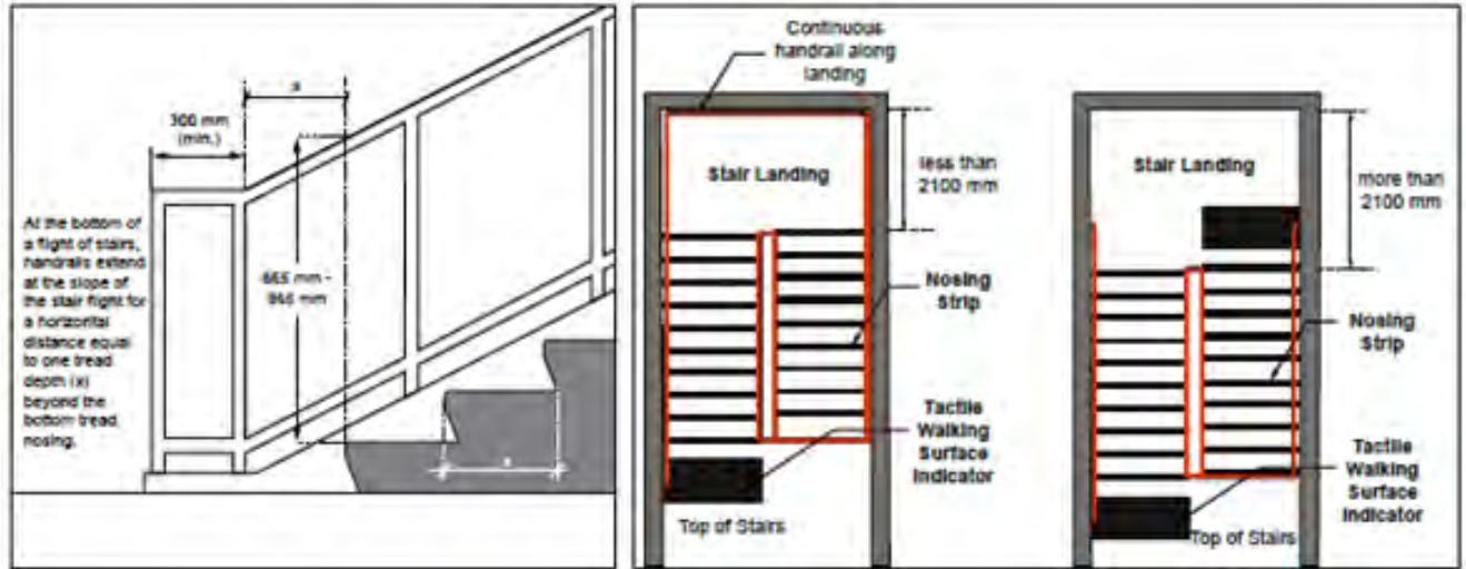
Figure 33: Stair shape
