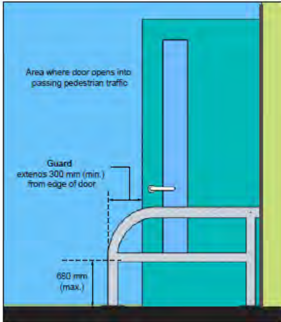
Figure 6: Example of a guard at door
