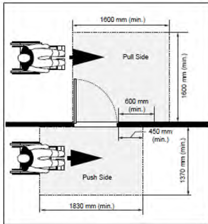
Figure 10: Side-Hinged Door - Hinge Side
