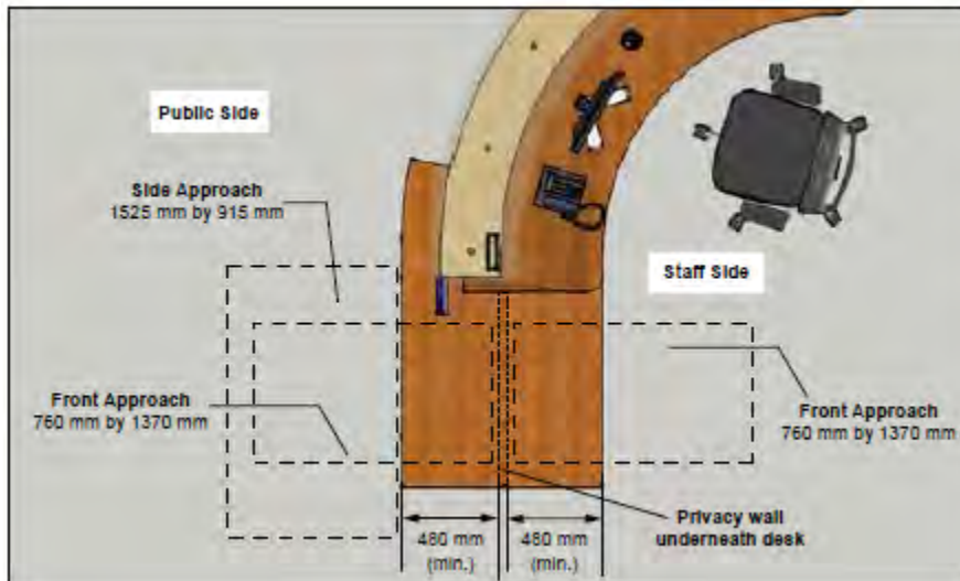
Figure 50: Accessible counter examples
