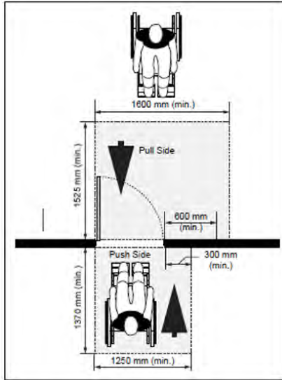
Figure 8: Side-Hinged Door - Front Approach
